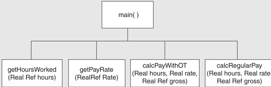
Figure 4-10 Hierarchy chart
