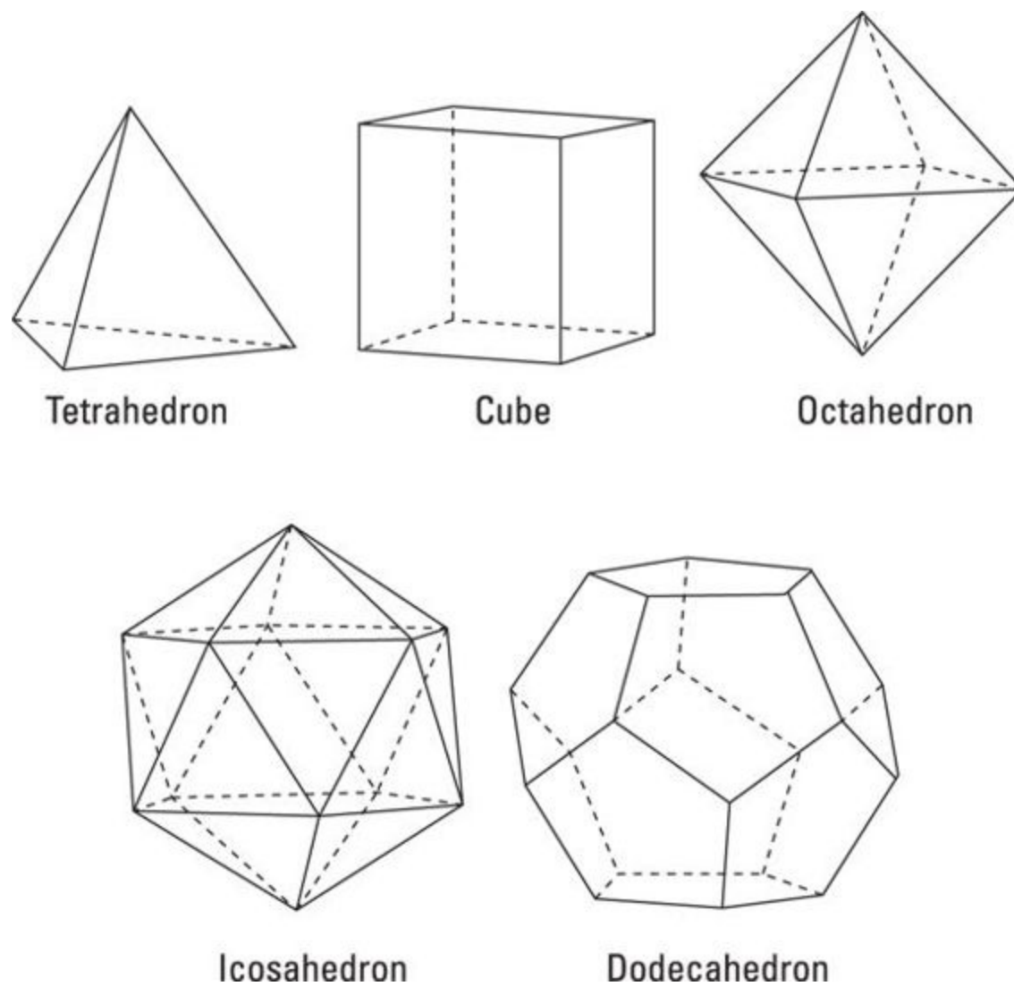
FIGURE 16-8: The five regular solids.
