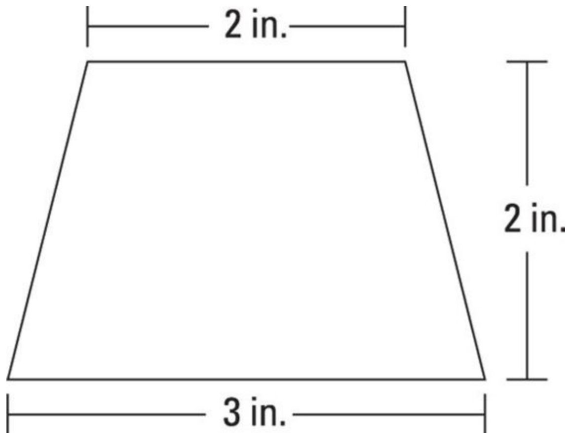
FIGURE 16-14: Measuring a trapezoid.
