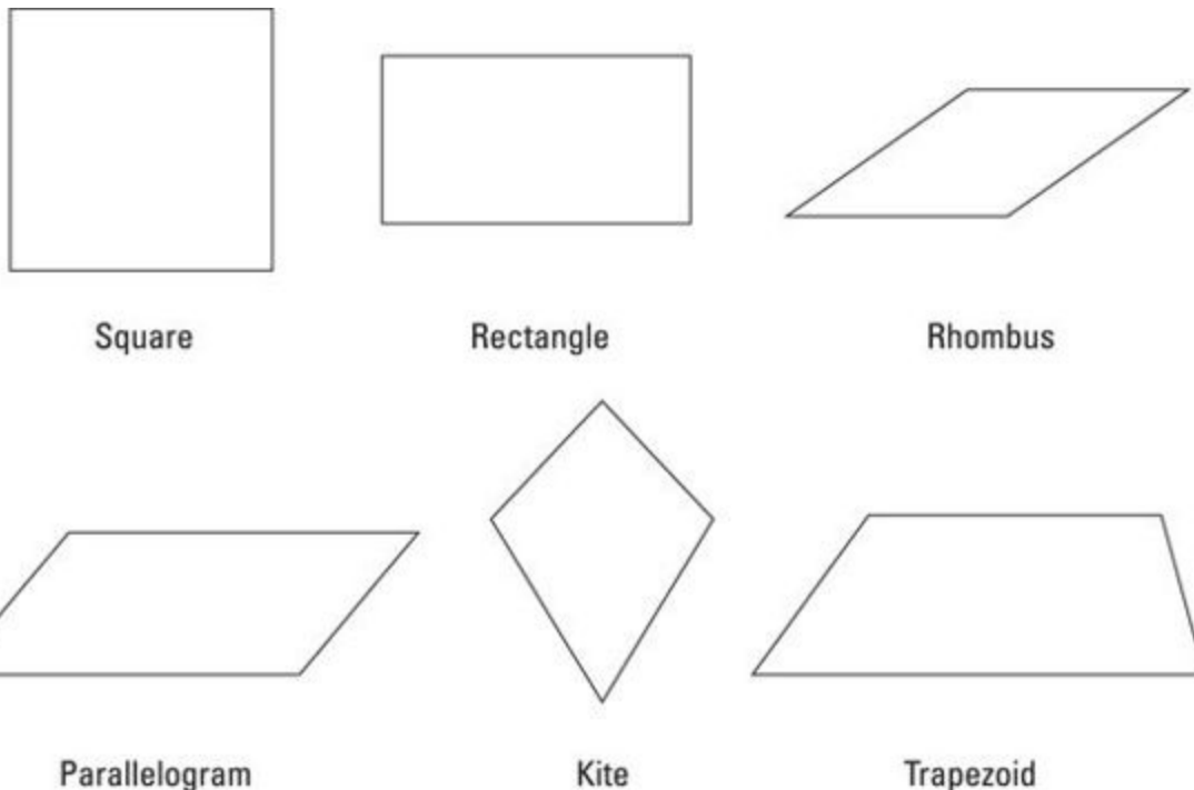
FIGURE 16-3: Common quadrilaterals.
