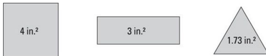
FIGURE 16-11: The areas of figures.
