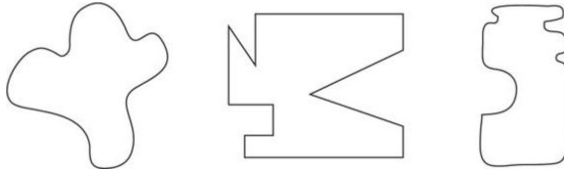
FIGURE 16-1: Unnamed shapes.
