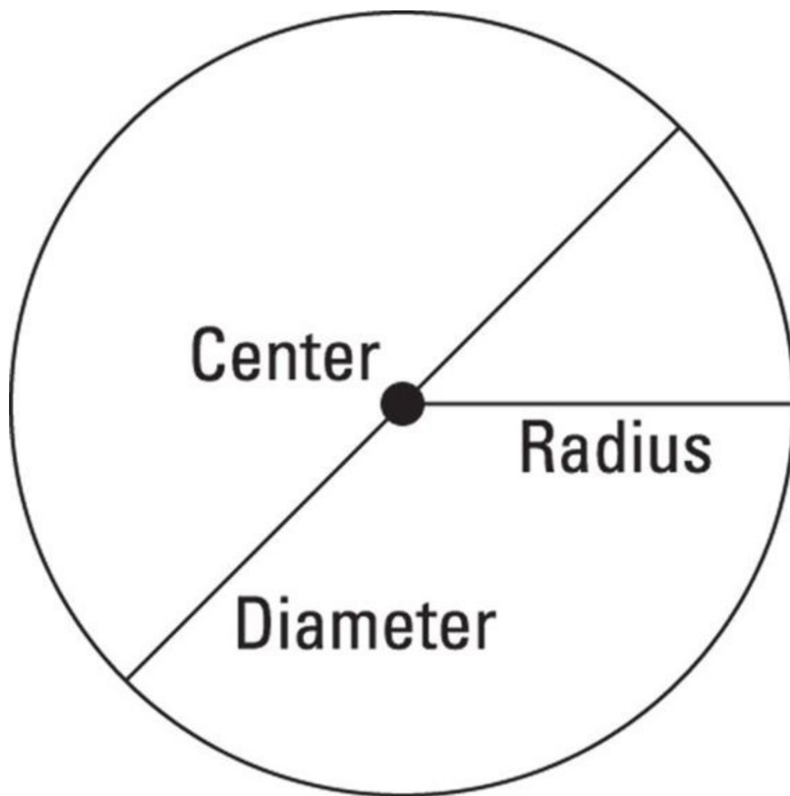
FIGURE 16-17: Deciphering the parts of a circle.
