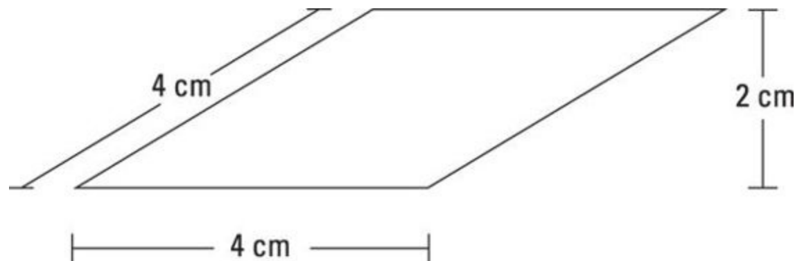
FIGURE 16-12: Measuring a rhombus.
