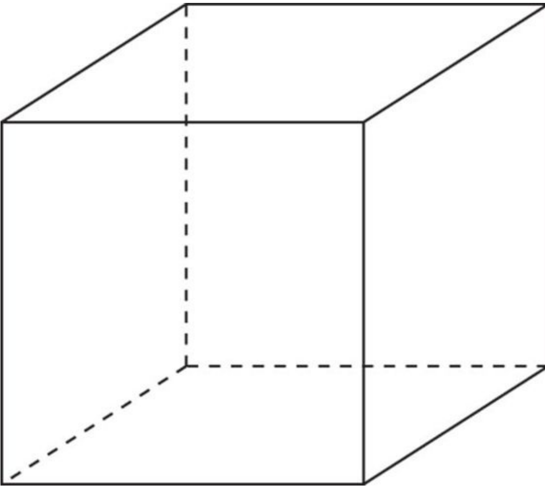
FIGURE 16-6: A typical cube.
