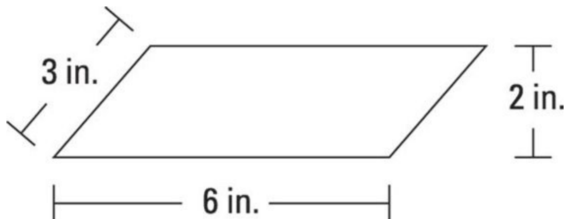
FIGURE 16-13: Measuring a parallelogram.
