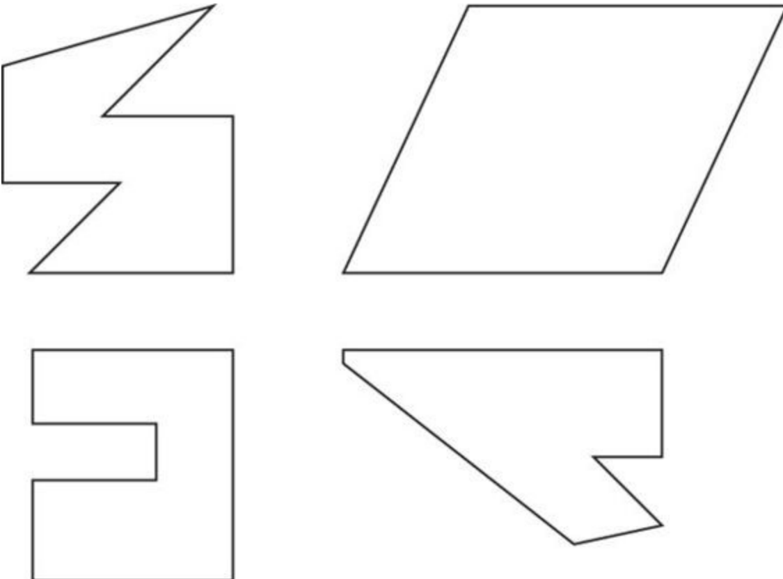
FIGURE 16-5: Various irregular polygons.
