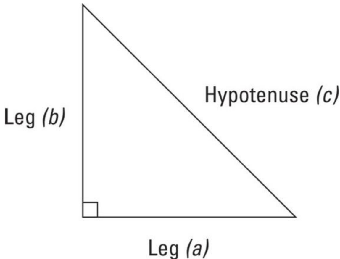
FIGURE 16-16: The hypotenuse and legs of a right triangle.
