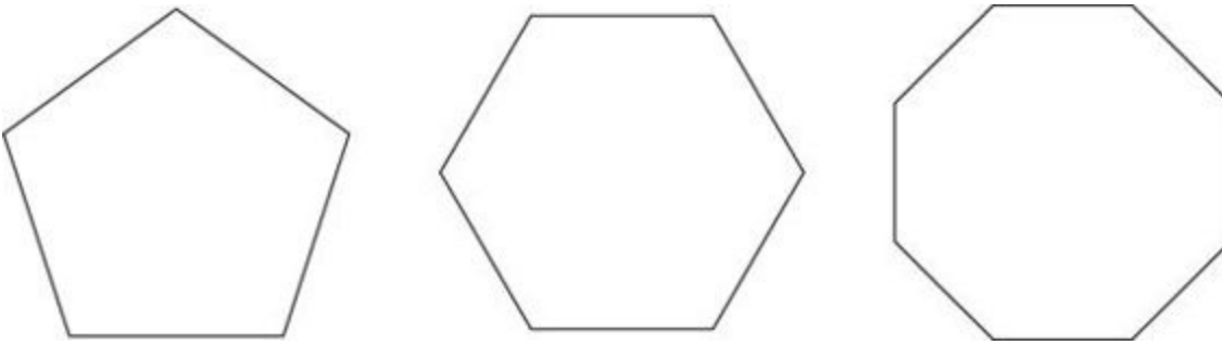
FIGURE 16-4: A pentagon, a hexagon, and an octagon.
